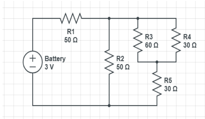
Circuit 2
